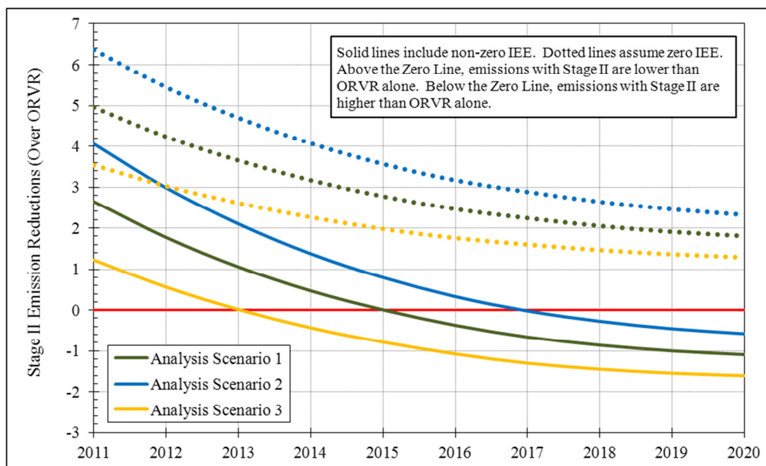
Figure 3. Results Set 3 – Onroad+Nonroad, Displacement Impacts Only (VOC, metric tonnes per day)
